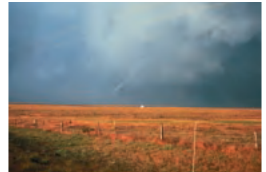
Figure 20: Tornado in its dissipating stage. Photo - Courtesy Gary Woodall.
