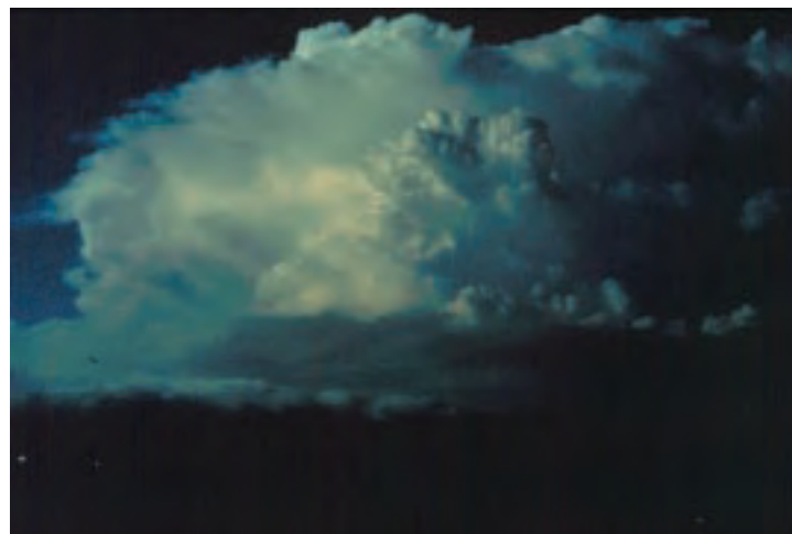
Figure 9: Non-severe multicell storm. Photo - NSSL.
