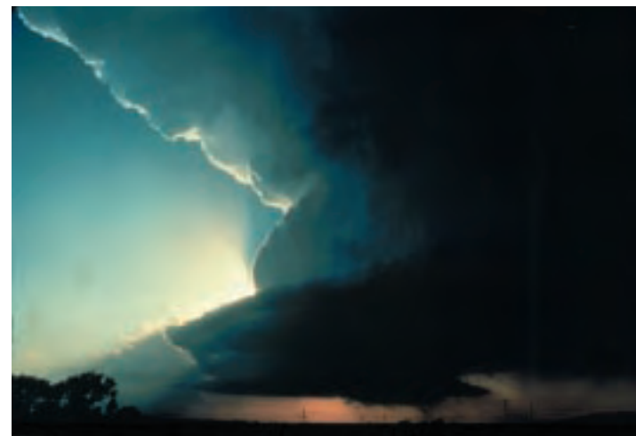
Figure 32: Side view of an LP supercell. Photo - NSSL.
